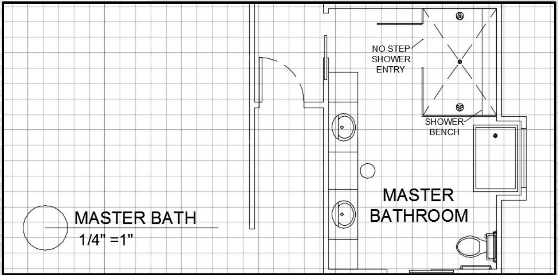
Floor Plan
